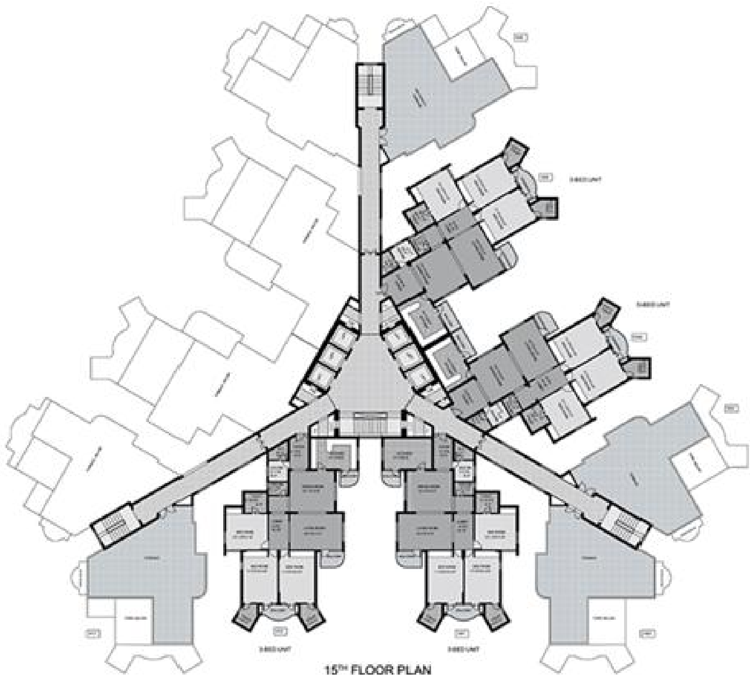
15 TH FLOOR PLAN
