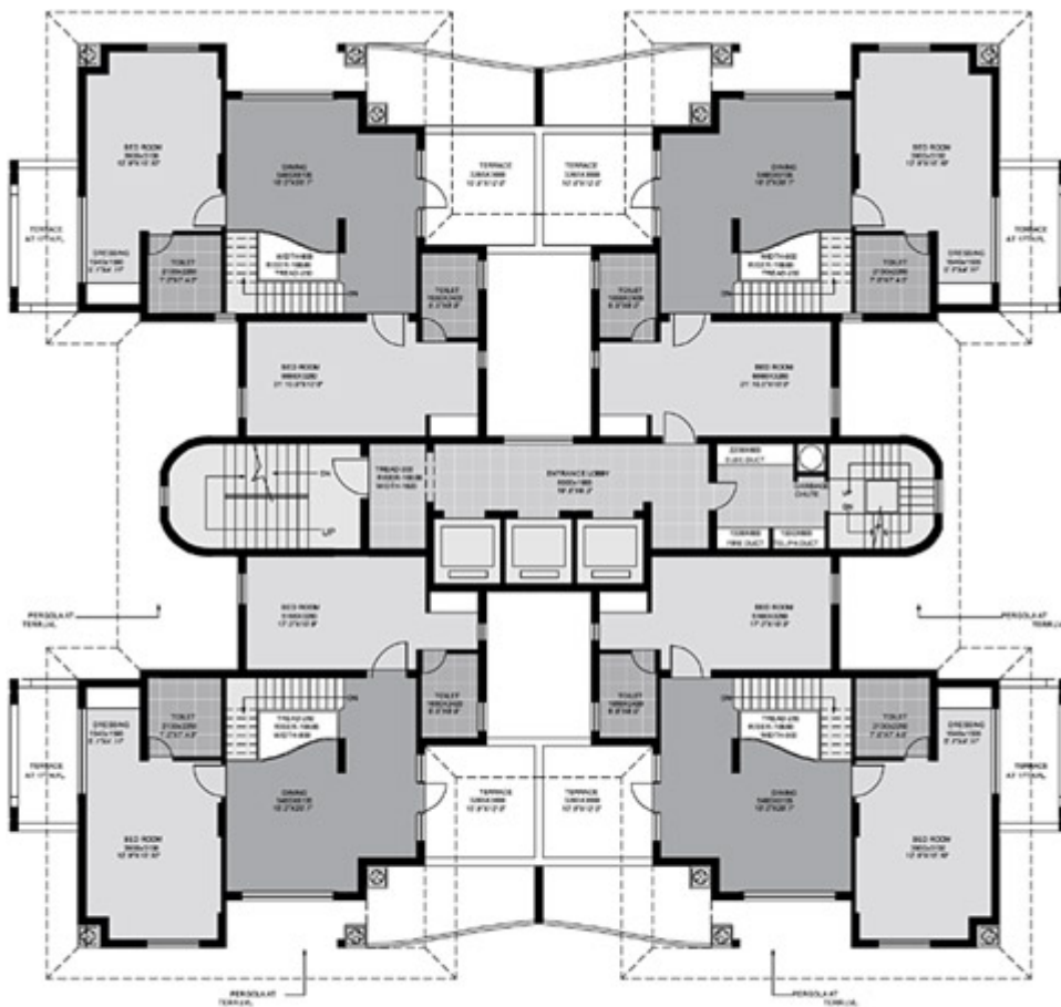
17 TH FLOOR PLAN (UPPER DUPLEX)
