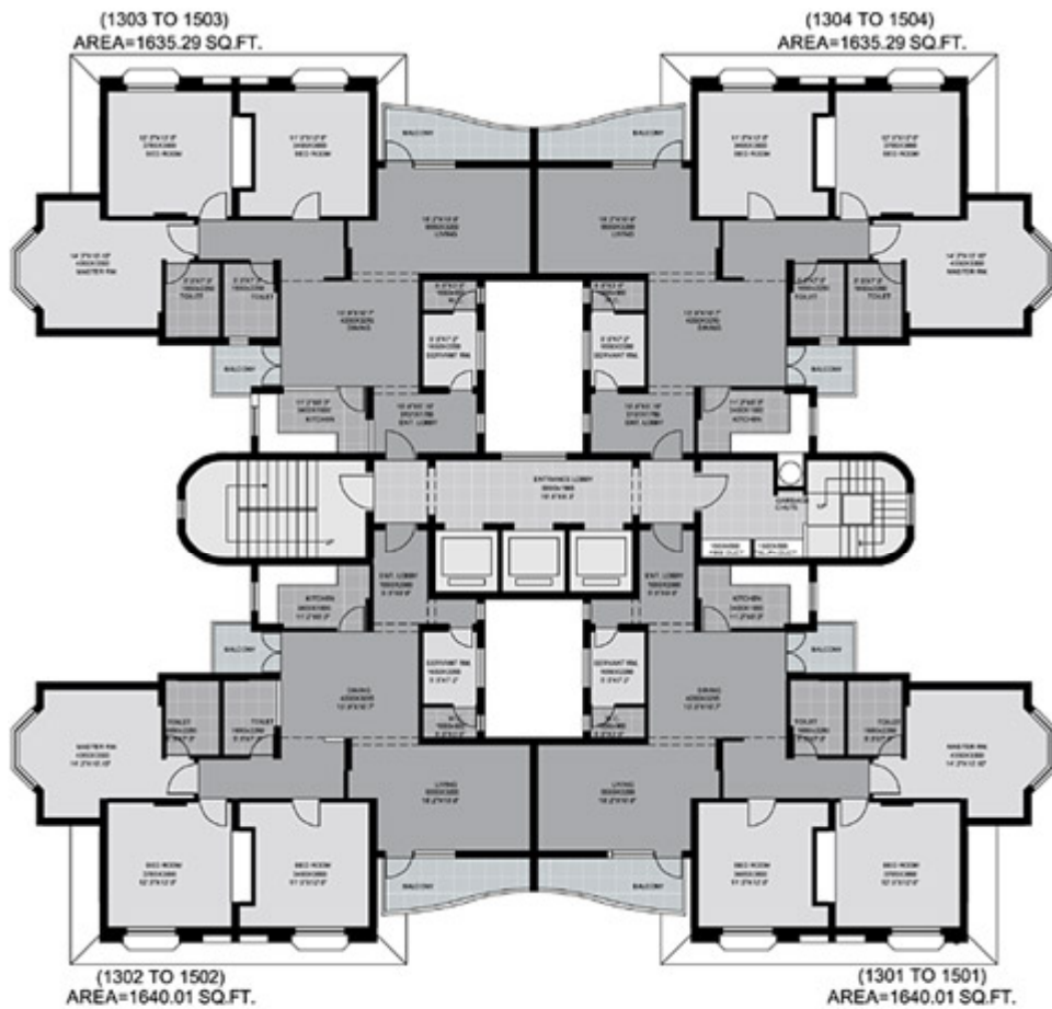
13TH TO 15TH FLOOR PLAN
