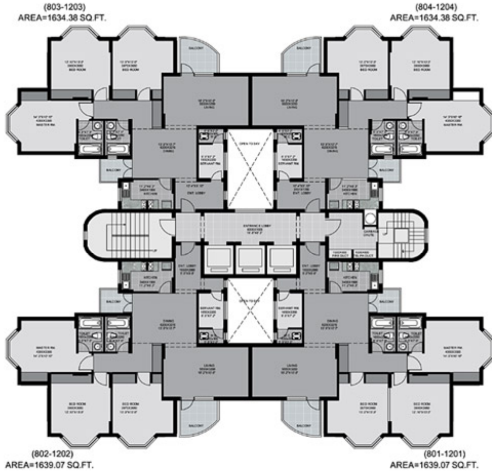
8 TH TO 12 TH FLOOR PLAN
