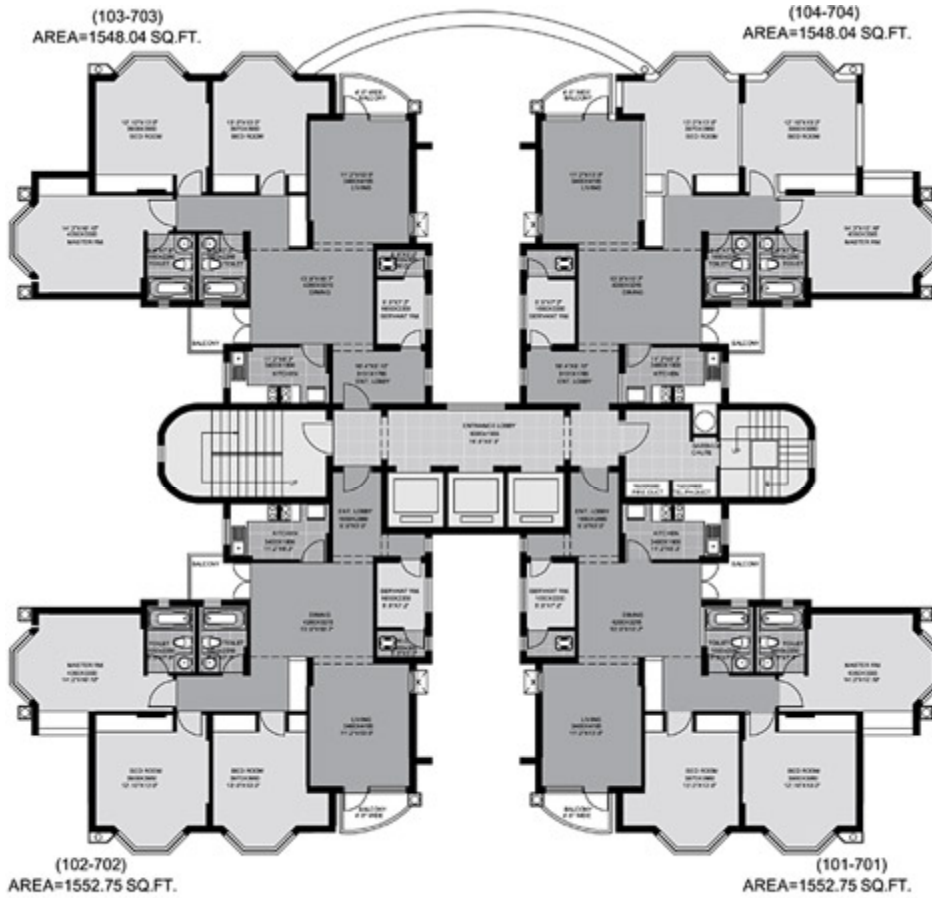
1 ST TO 7 TH FLOOR PLAN
