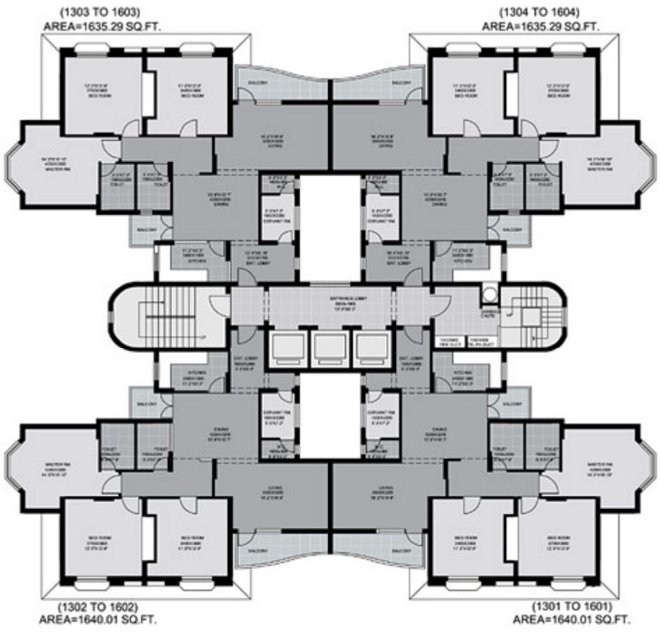
13 TH TO 16 TH FLOOR PLAN
