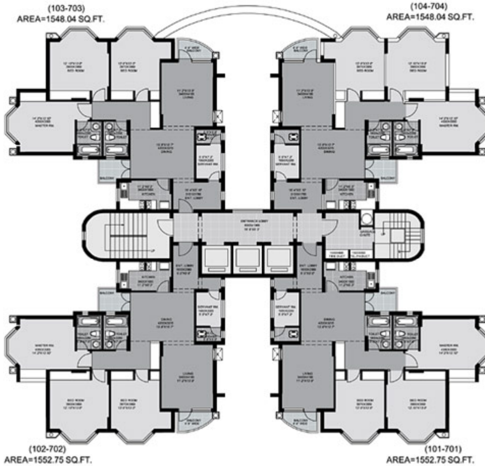
1 st TO 7 th FLOOR PLAN
