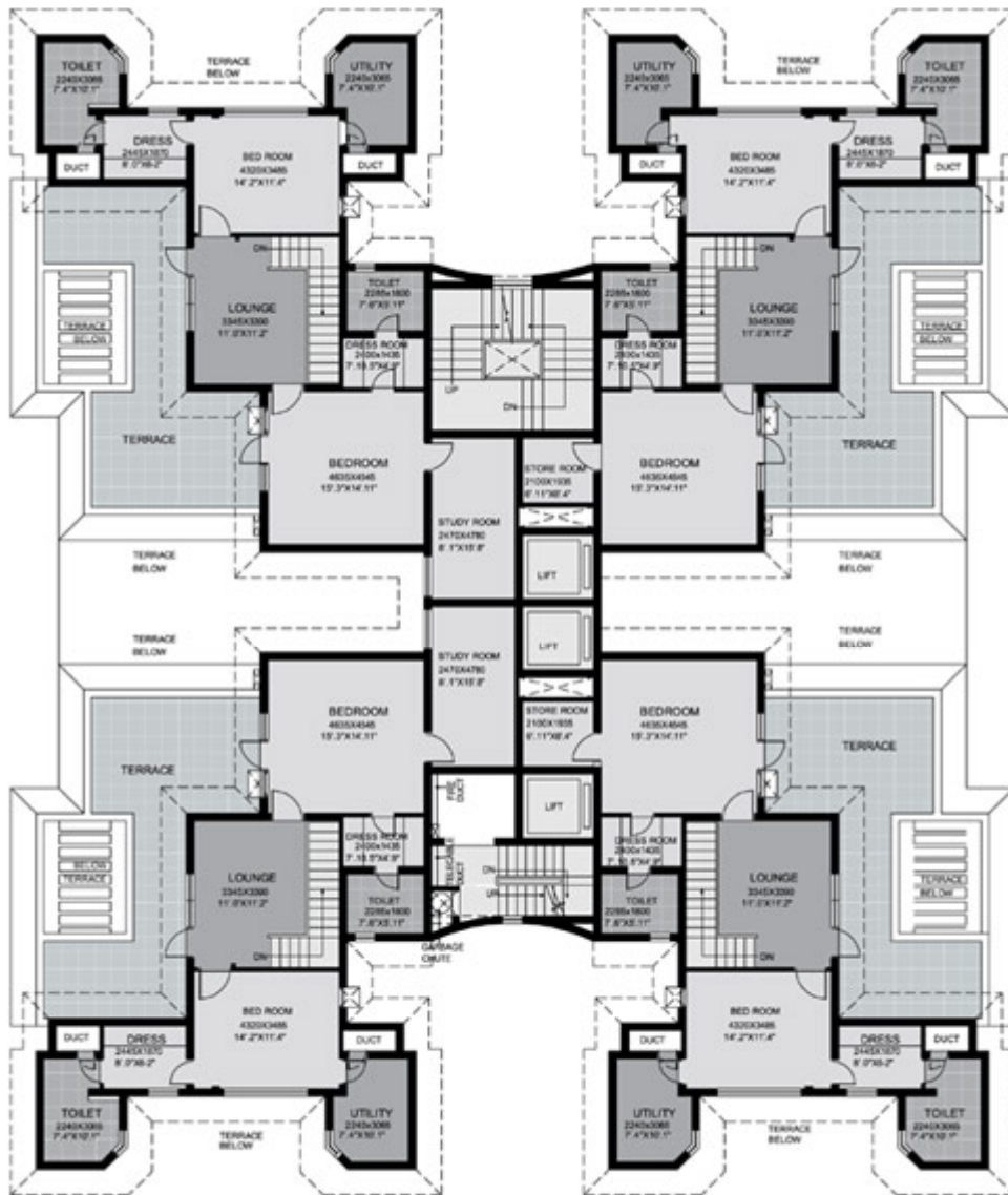
17 TH FLOOR PLAN (UPPER DUPLEX)
