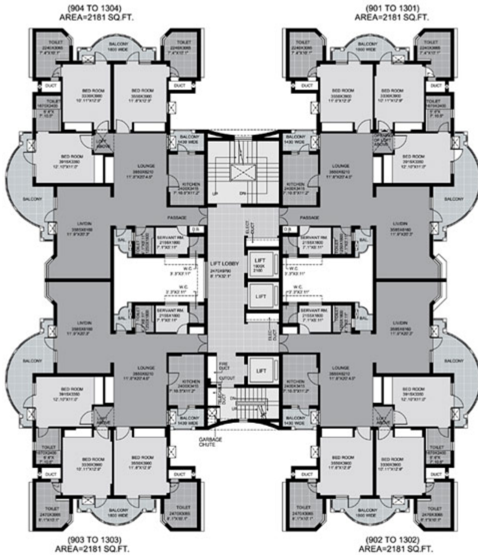
9 TH TO 13 TH FLOOR PLAN
