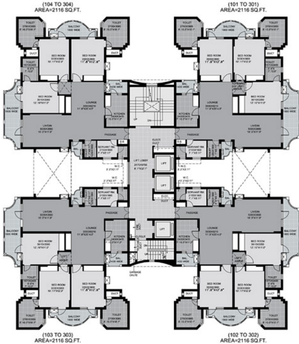
1 ST TO 3 RD FLOOR PLAN
