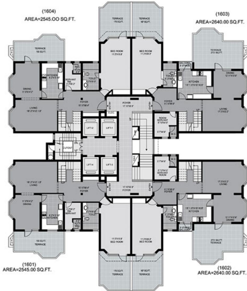
16 TH FLOOR PLAN (LOWER DUPLEX)
