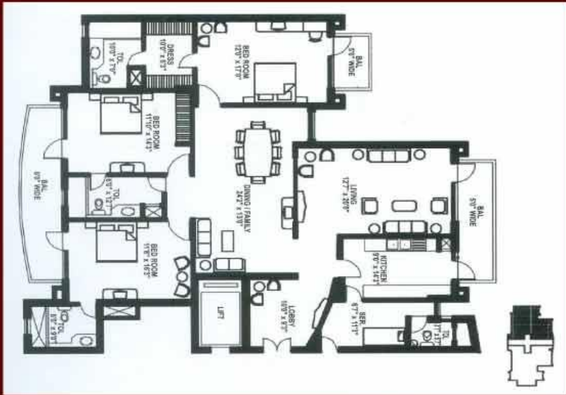
Ground and First Floor Plan 3- Bedroom Unit
