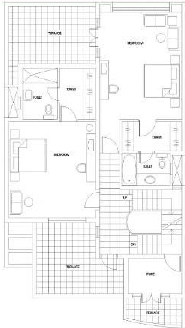
Coral Court : Second Floor Plan
