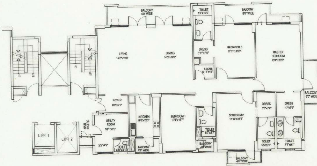
6 SECOND,THIRD FLOOR PLAN
