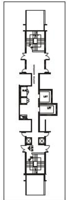
CORE PLAN
