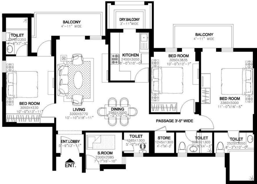
TENTATIVE PLAN OF APARTMENT NO. 1, 2 & 4 IN BLOCK B, E & H TENTATIVE PLAN OF APARTMENT NO. 1 IN BLOCK A, C, D, F, G, J, K & L
